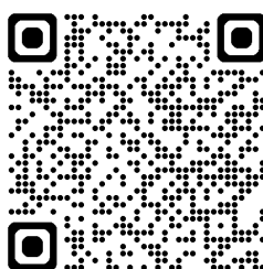
waves
