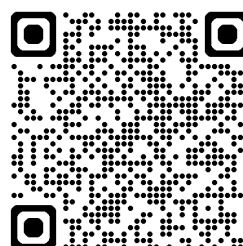
atomic structure
